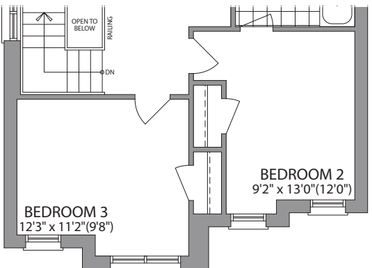
SECOND FLOOR ELEVATION B
