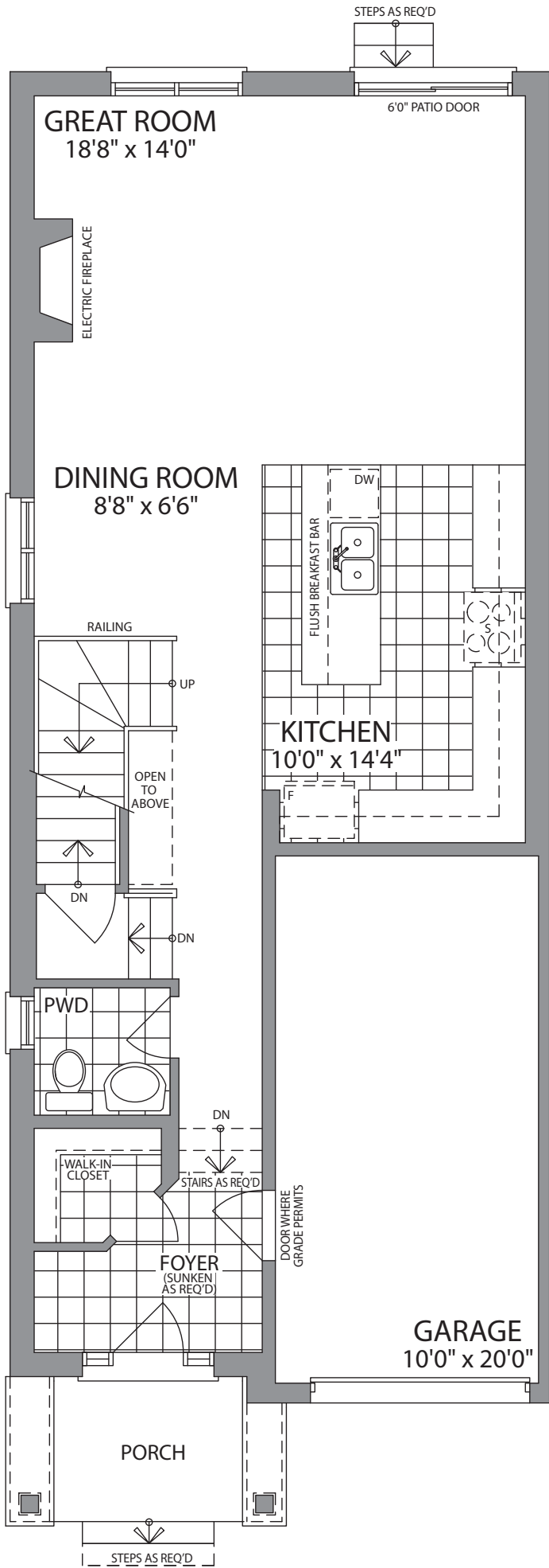
GROUND FLOOR ELEVATION A
