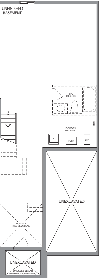
BASEMENT ELEVATION A & B
