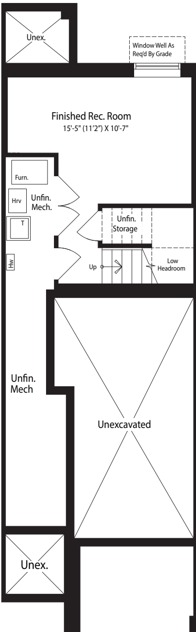
Finished Lower Floor Plan Elevations 'A1', 'B1'
