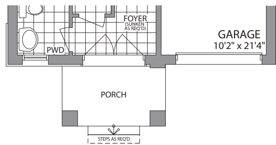
GROUND FLOOR ELEVATION C
