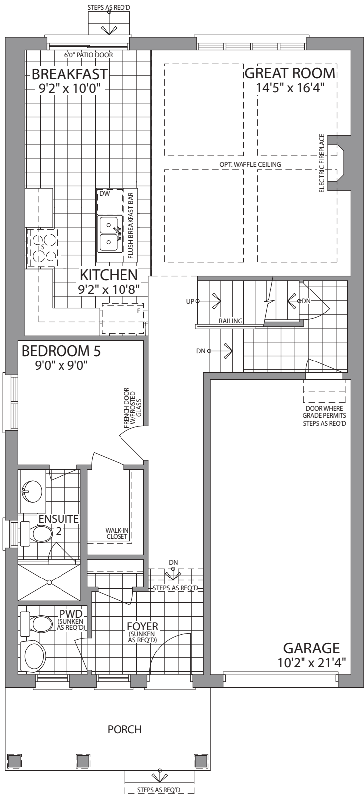
OPT. GROUND FLOOR W/5 BEDROOMS ELEVATION A
