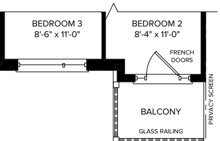
PARTIAL THIRD FLOOR ELEVATION B
