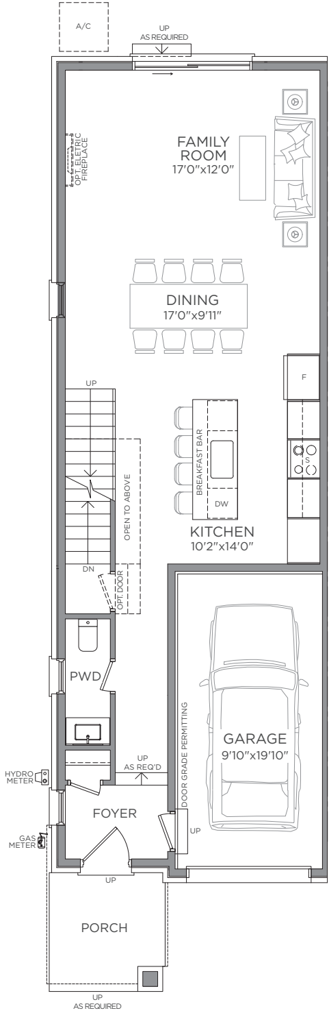
MAIN FLOOR PLAN
