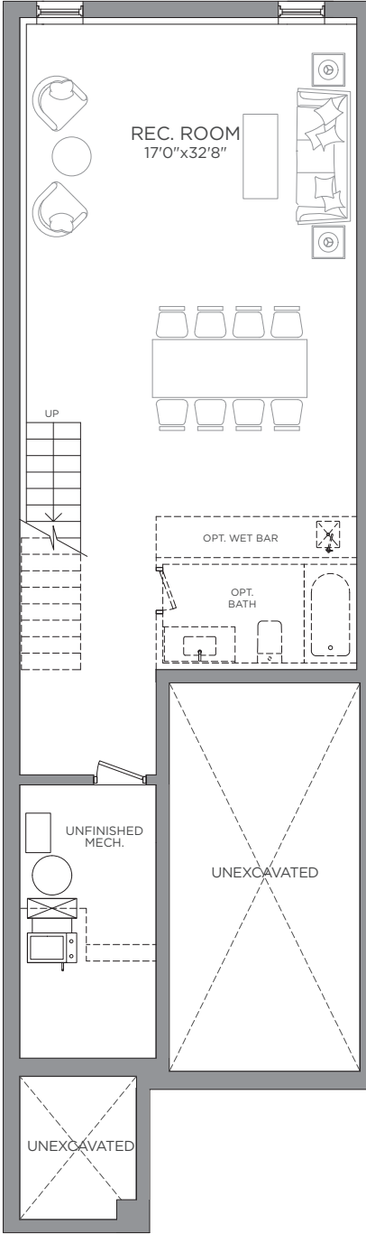
BASEMENT FLOOR PLAN FINISHED
