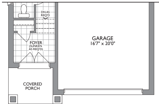
PARTIAL MAIN LEVEL ELEV. B & C
