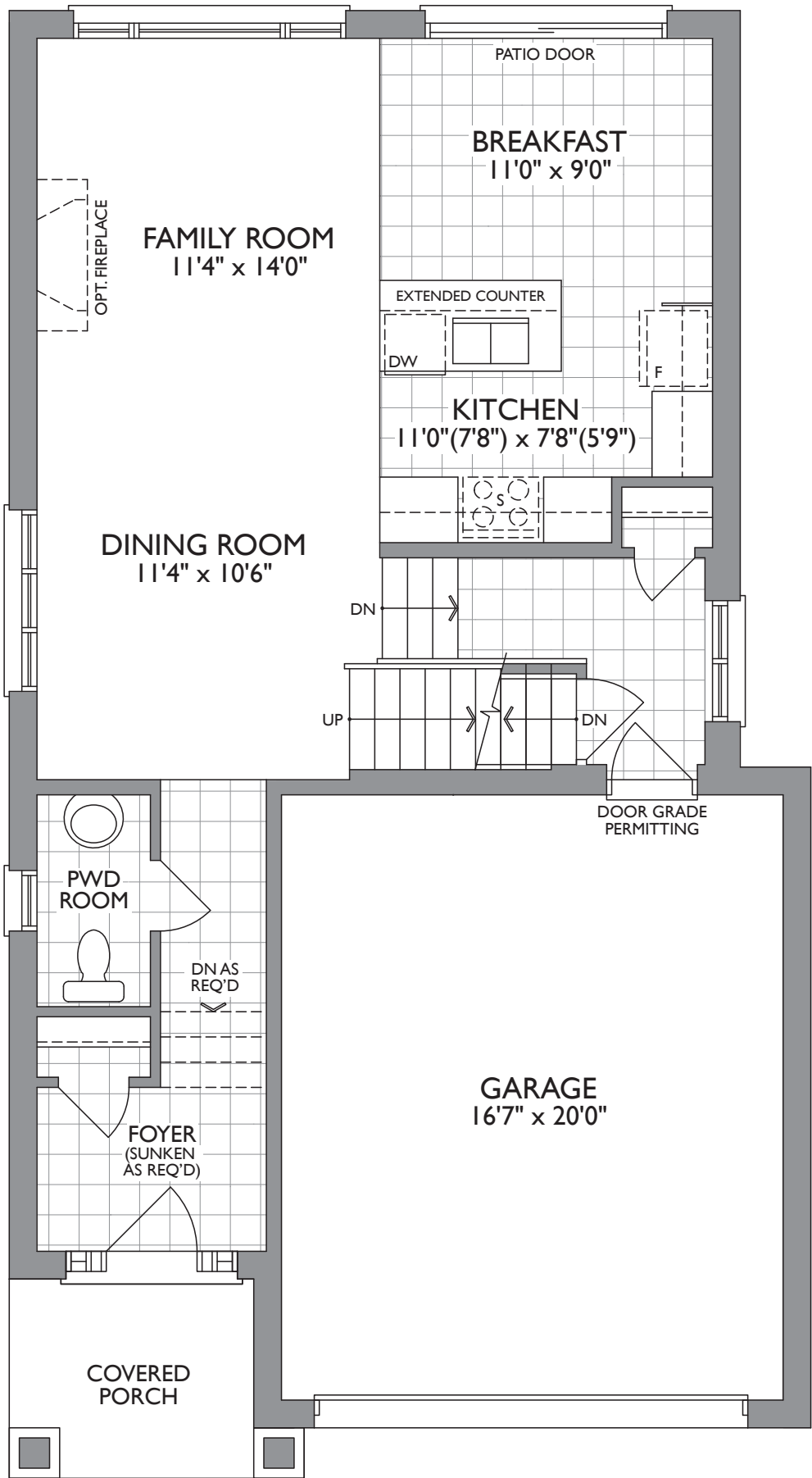
MAIN LEVEL ELEV. A
