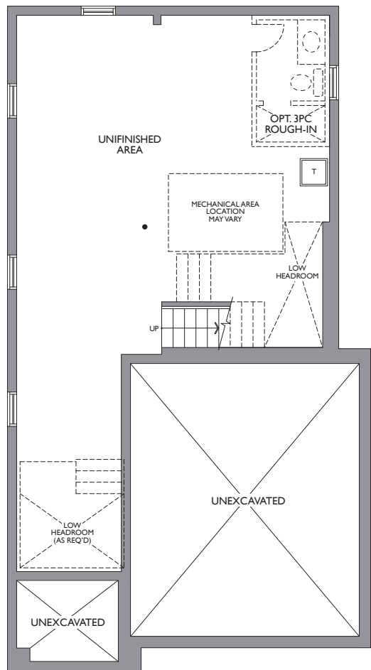
LOWER LEVEL ELEV. A, B & C
