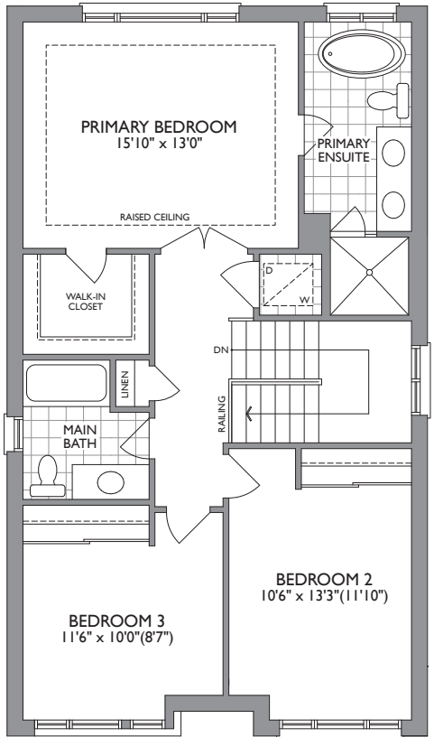
UPPER LEVEL ELEV. B
