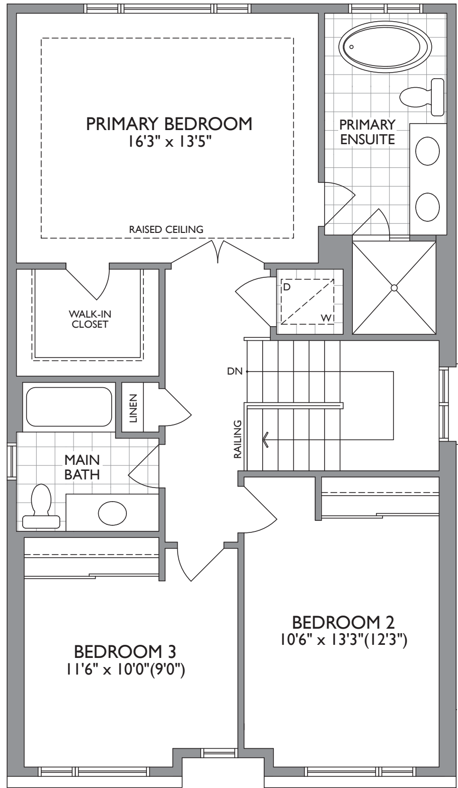
UPPER LEVEL ELEV. A
