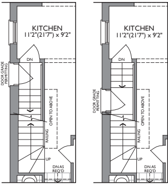
PARTIAL MAIN LEVEL WITH OPT. SIDE DOOR (LOCATION MAY VARY BASED ON GRADE) ELEV. A, B & C
