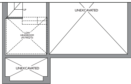
PARTIAL LOWER LEVEL ELEV. B
