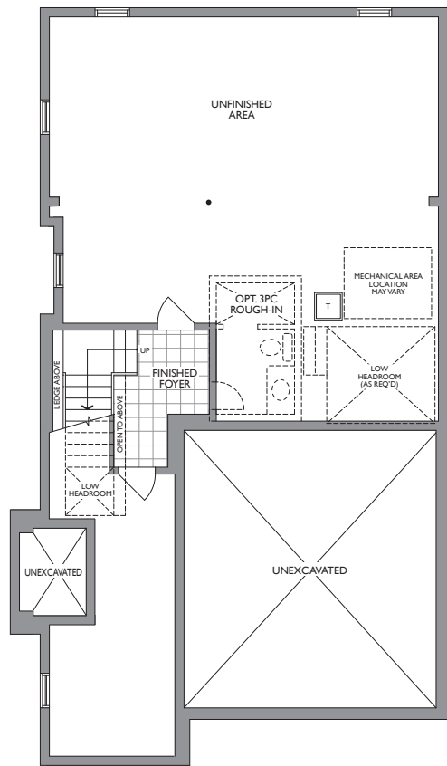
LOWER LEVEL ELEV. A & B
