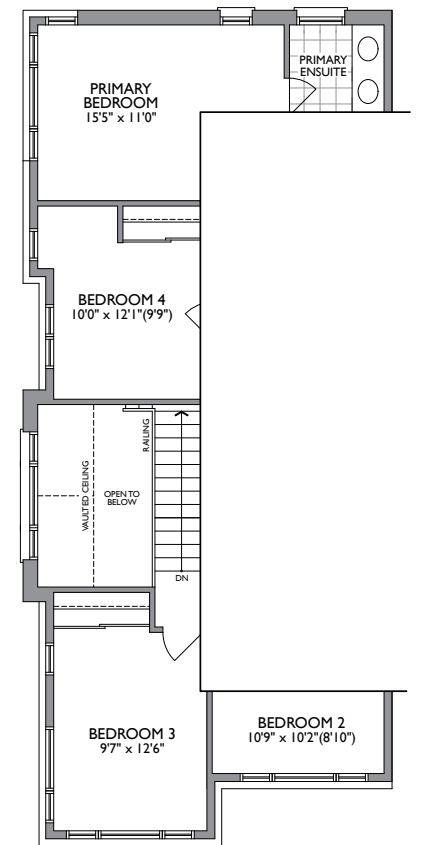
PARTIAL UPPER LEVEL ELEV. B
