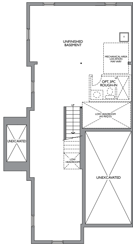
LOWER LEVEL ELEV. A
