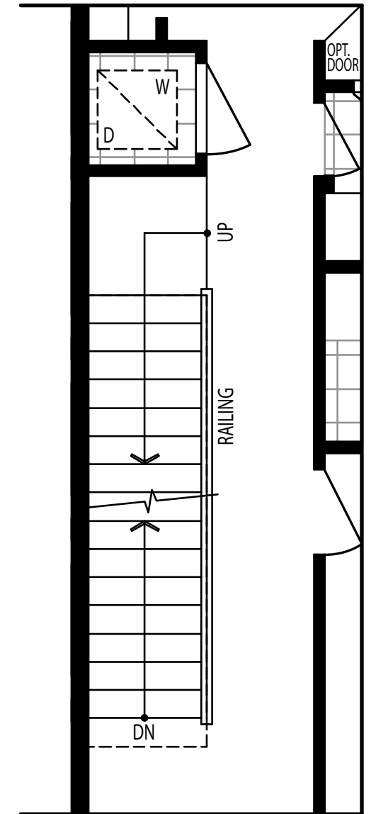
PARTIAL UPPER FLOOR PLAN FOR OPT. ROOF TERRACE ELEV. A1
