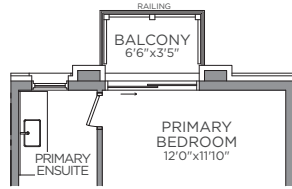
PART. UPPER FLOOR PLAN ELEV. B
