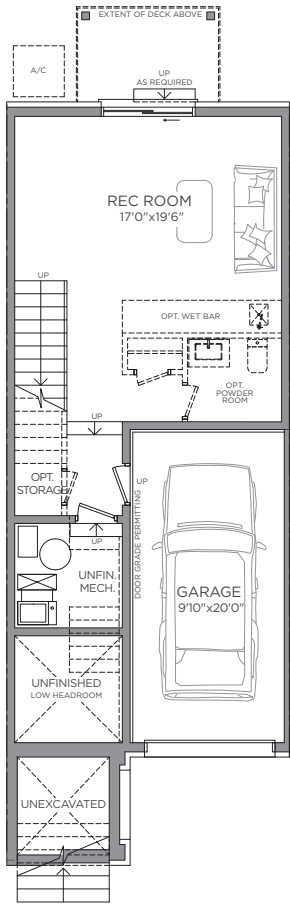
GROUND FLOOR PLAN ELEV. A FINISHED
