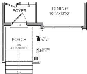
PART. MAIN FLOOR PLAN ELEV. B
