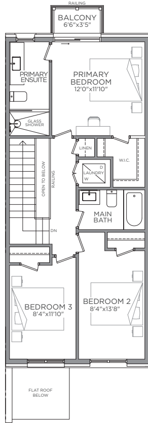
UPPER FLOOR PLAN ELEV. A
