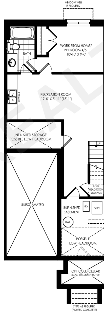
OPT. FINISHED BASEMENT ADDS 494 - 503 SQ.FT. ELEV. A
