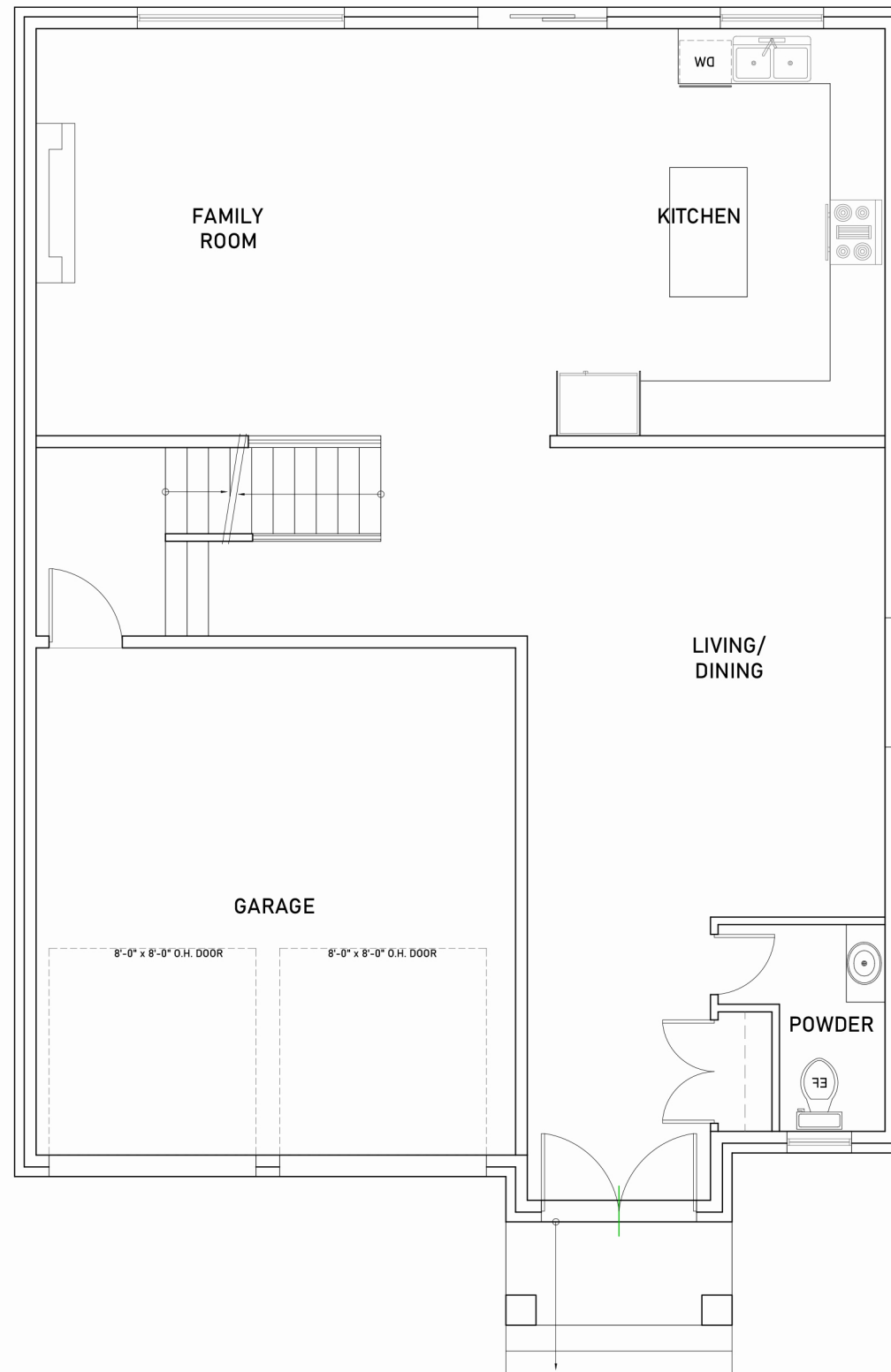
Main Floor
