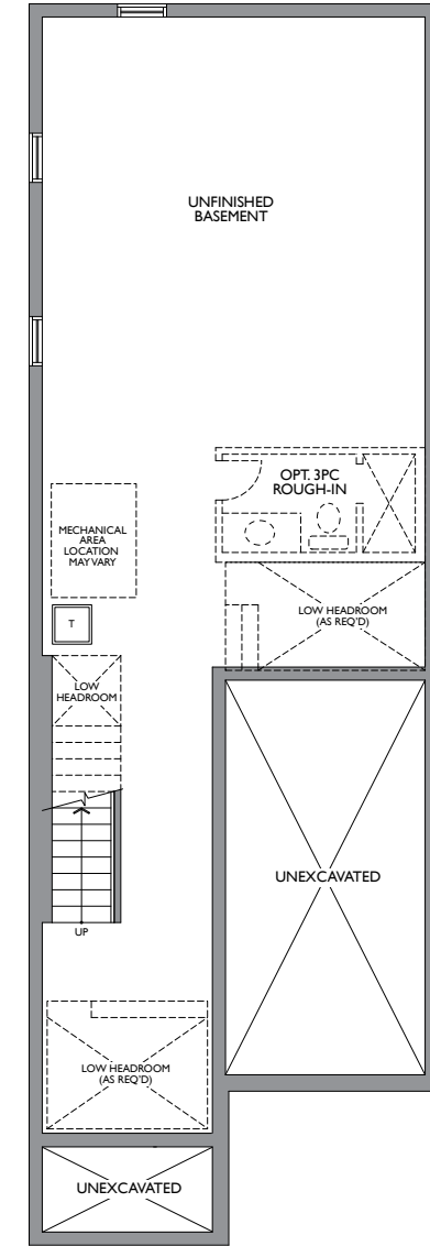
LOWER LEVEL ELEV. A
