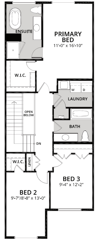
SECOND FLOOR
