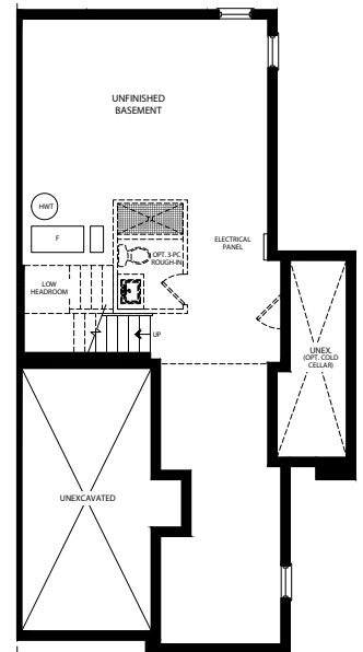
BASEMENT ELEV. A, B & C
