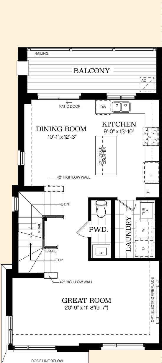
Main Floor Elevation A
