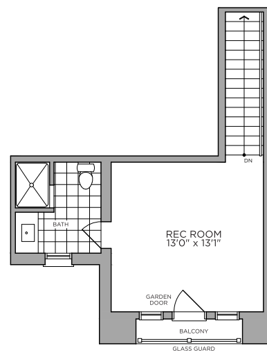
Third Floor ELEVATION A, B1
