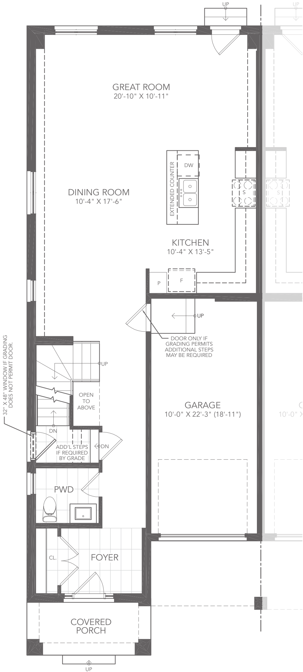
GROUND FLOOR PLAN A
