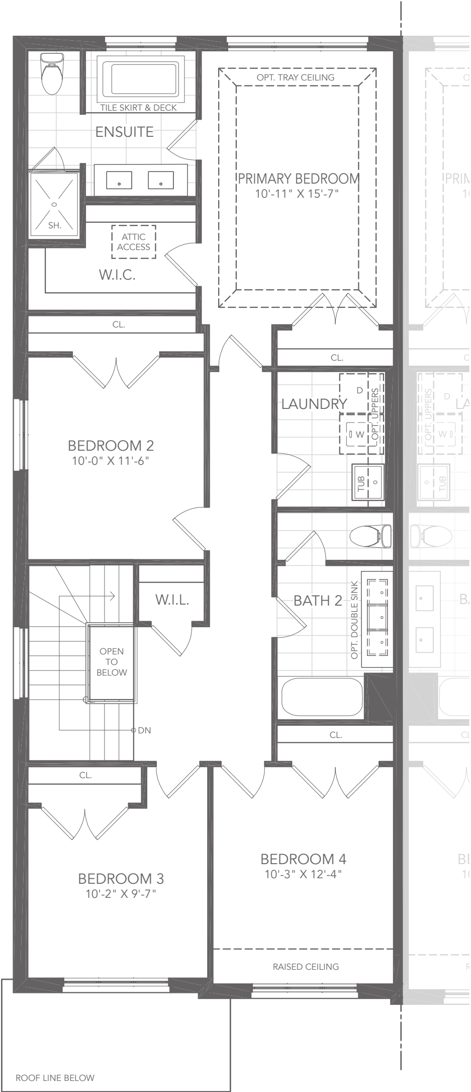
SECOND FLOOR PLAN A
