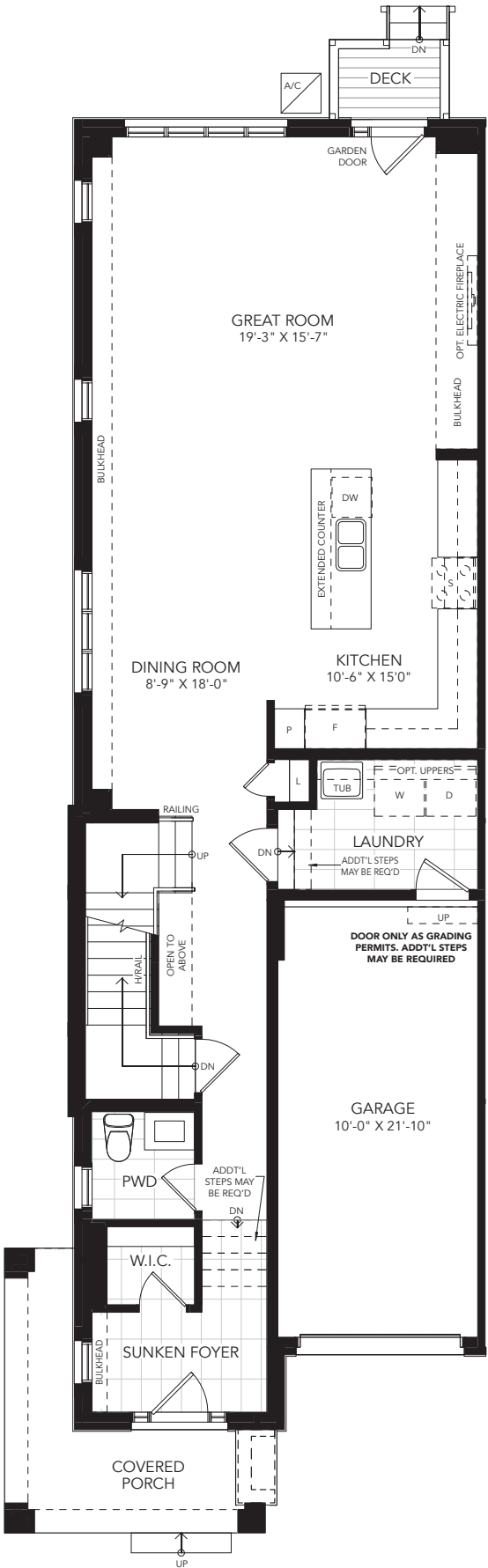
GROUND FLOOR PLAN ELEV. AA
