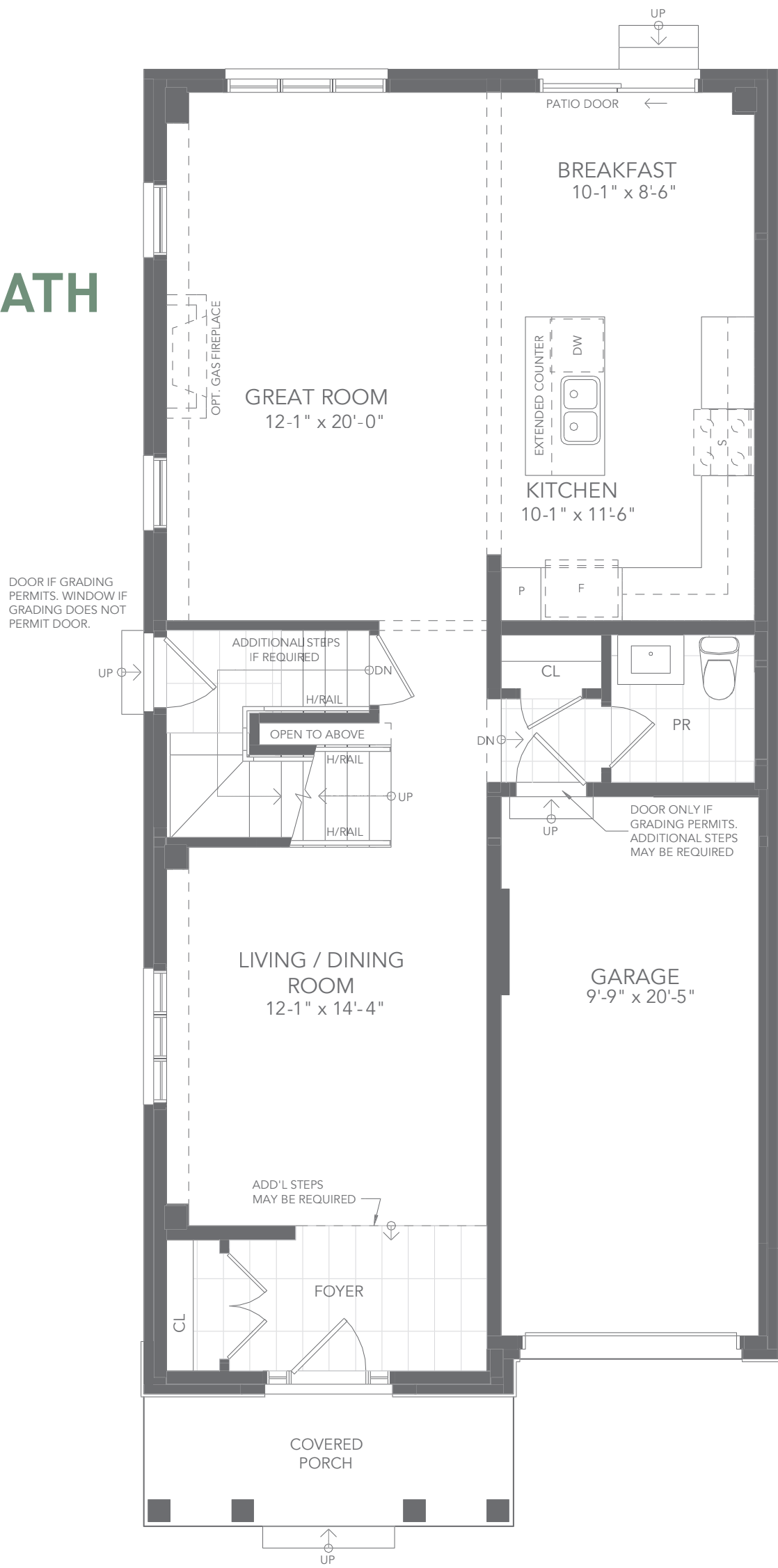
GROUND FLOOR PLAN A
