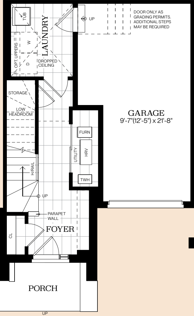
Lower Floor Elevation A
