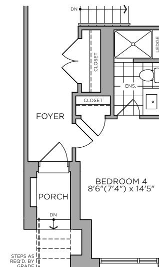
Optional First Floor BEDROOM 4 - ELEVATION A, B
