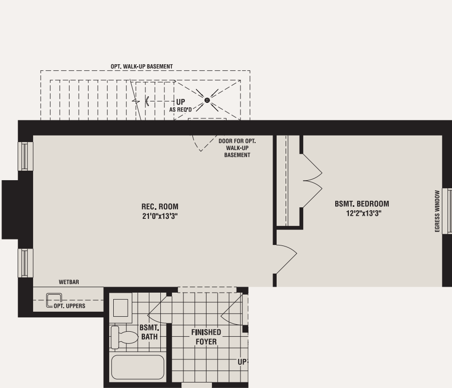
FAMILY FLEX SUITE OPTION
