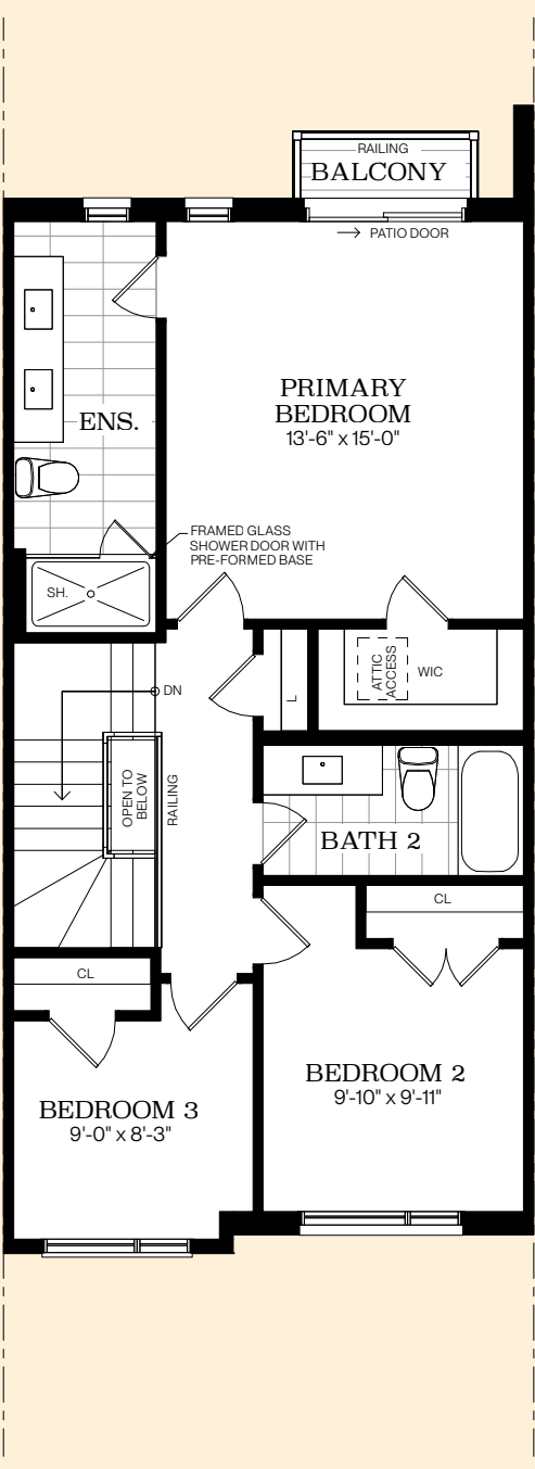
Upper Floor Elevation A
