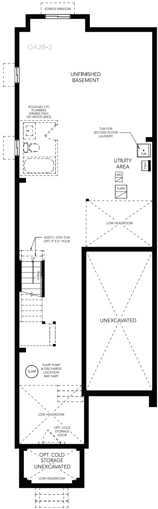
BASEMENT PLAN ELEV. A
