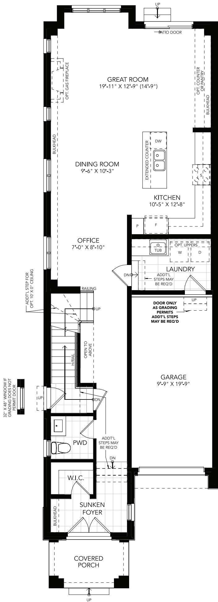
GROUND FLOOR PLAN ELEV. A
