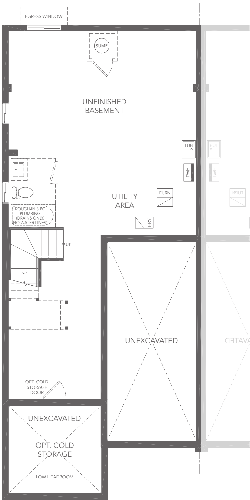
BASEMENT PLAN A
