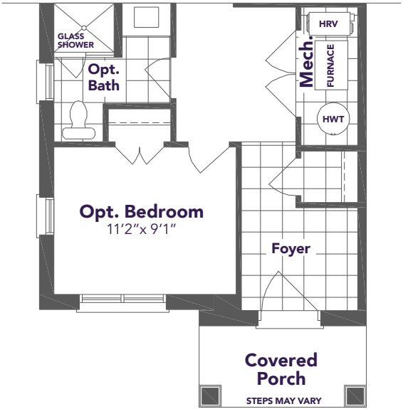
OPTIONAL GROUND FLOOR PLAN W/ OPTIONAL BEDROOM
