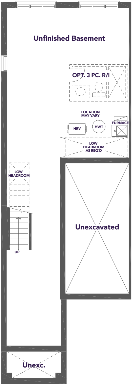
BASEMENT PLAN
