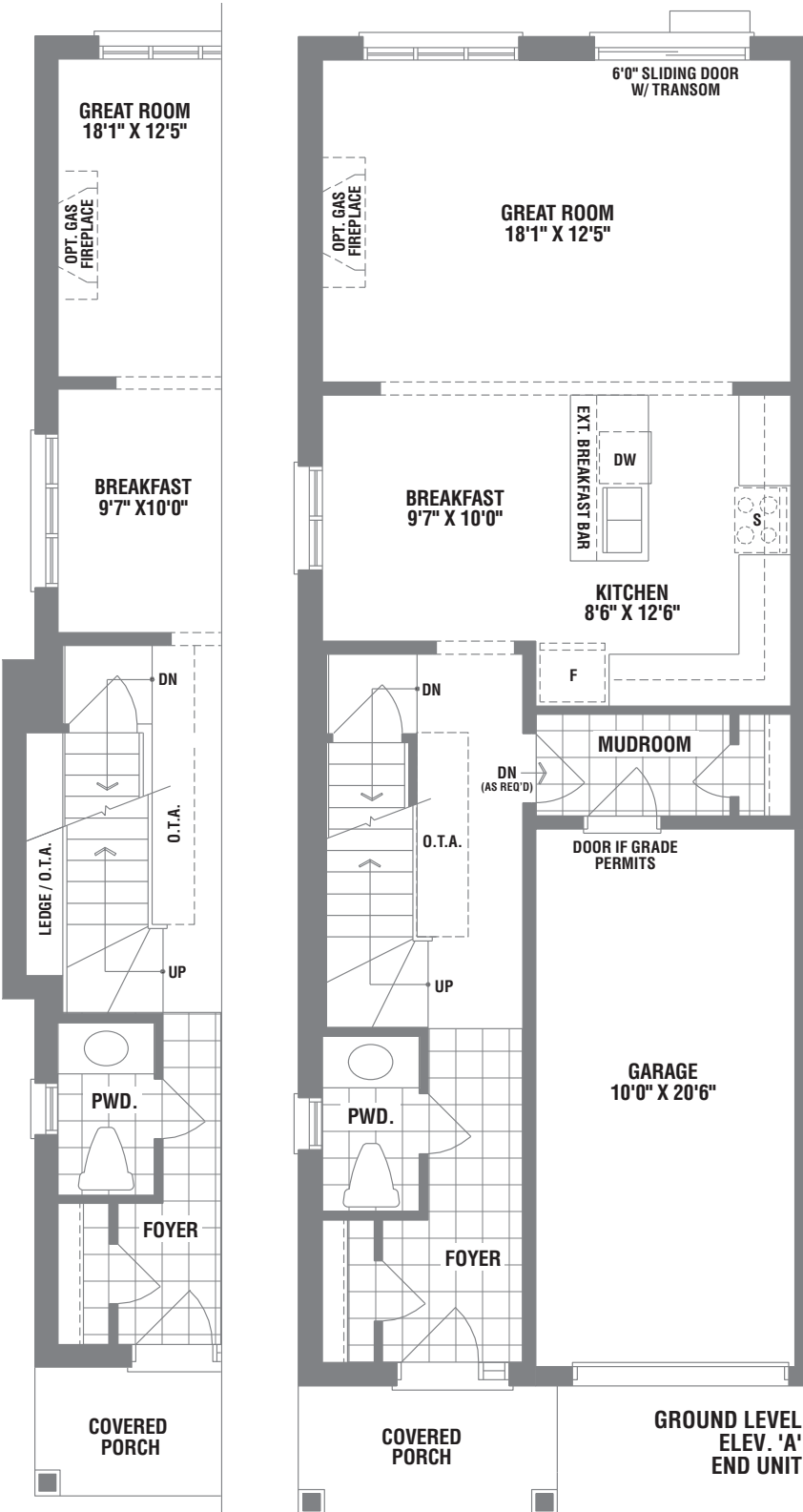
PART. GROUND LEVEL ELEV. 'A' & 'B' CORNER UNIT
