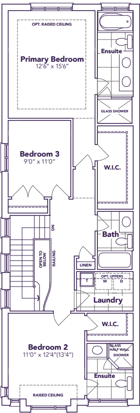
OPT. SECOND FLOOR
