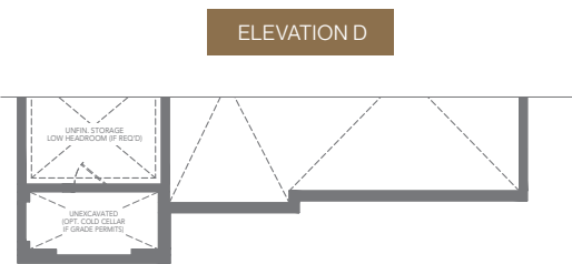
BASEMENT PLAN
