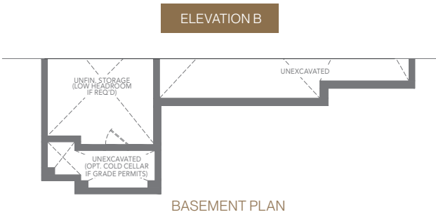
BASEMENT PLAN
