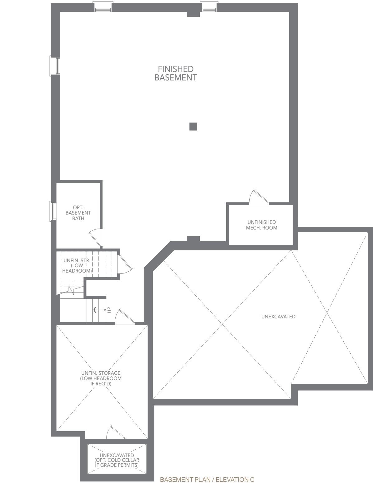
BASEMENT PLAN / ELEVATION C
