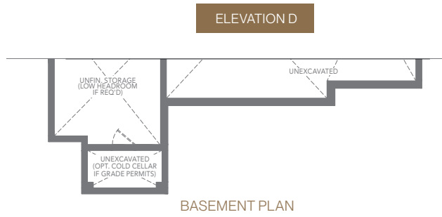
BASEMENT PLAN
