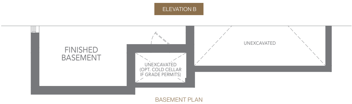
BASEMENT PLAN
