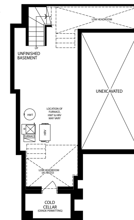
BASEMENT ELEV. A
