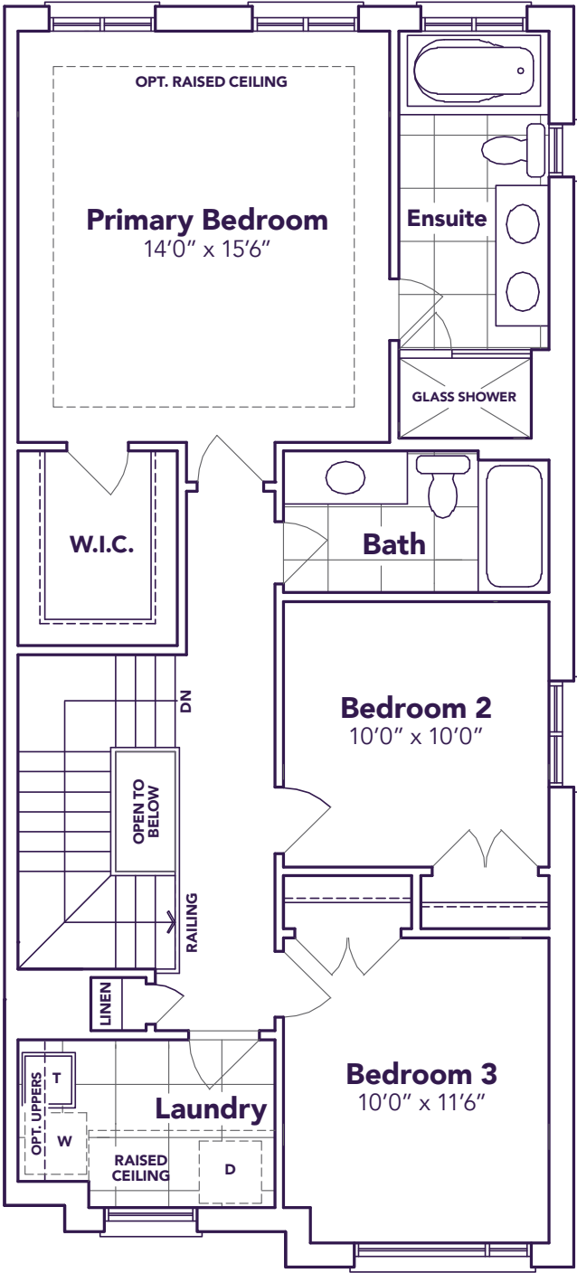
ELEVATION B1 SECOND FLOOR
