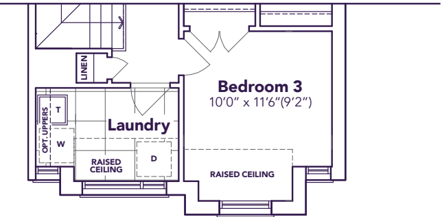
ELEVATION B2 PARTIAL SECOND FLOOR
