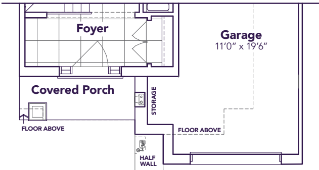
ELEVATION B2 PARTIAL MAIN FLOOR
