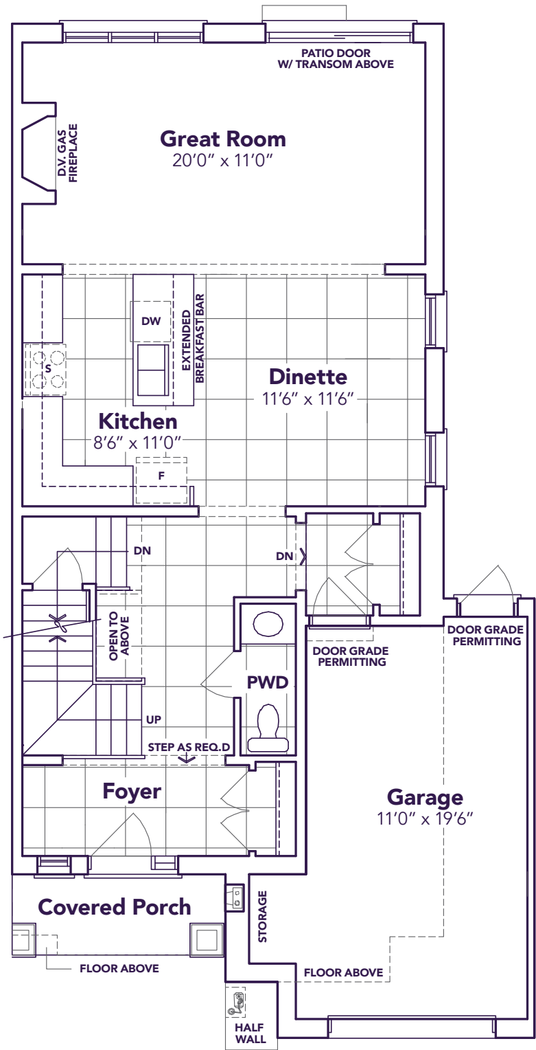
ELEVATION B1 MAIN FLOOR
