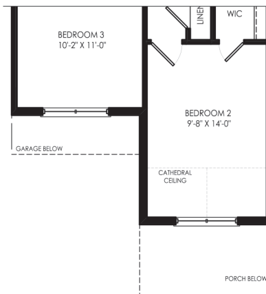
ELEVATION A2 SECOND LEVEL
