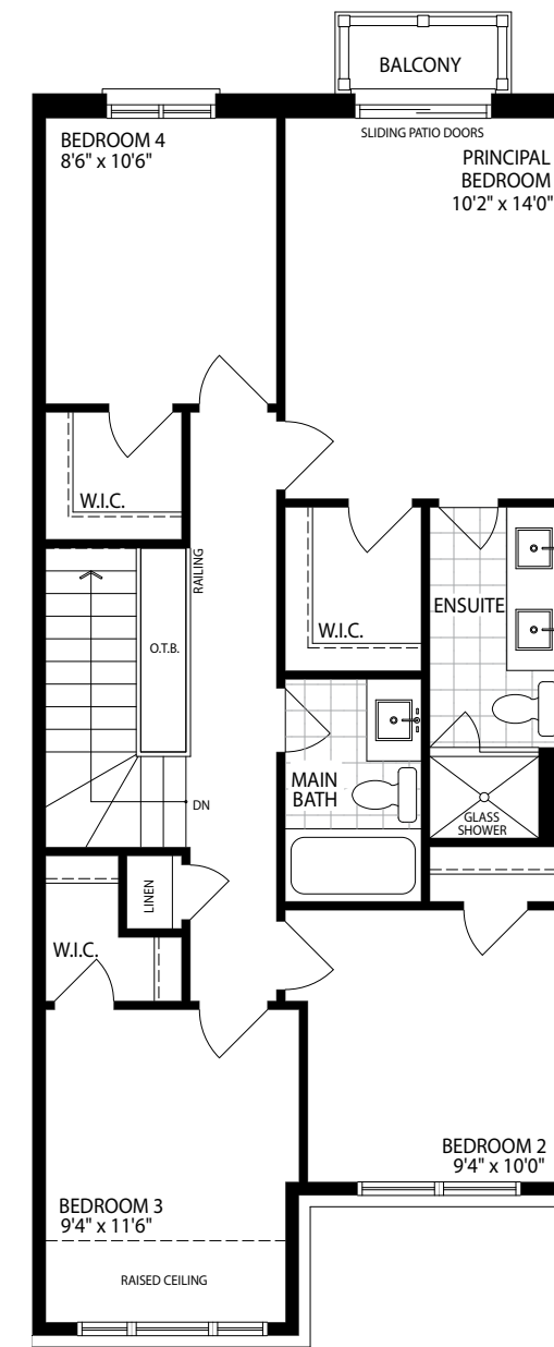
OPT. UPPER FLOOR WITH 4 BEDROOMS ELEV. A
