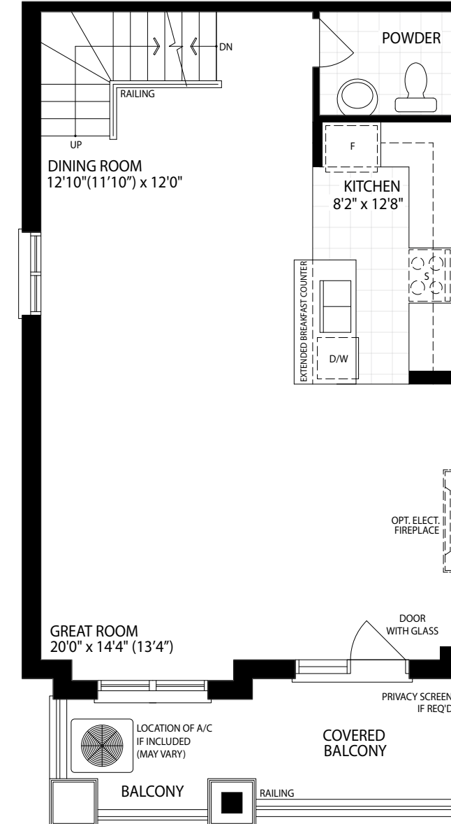
MAIN FLOOR ELEV. A
