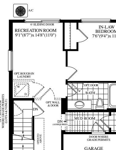
OPT. GROUND LEVEL ELEVATION A & B (IN-LAW SUITE)
