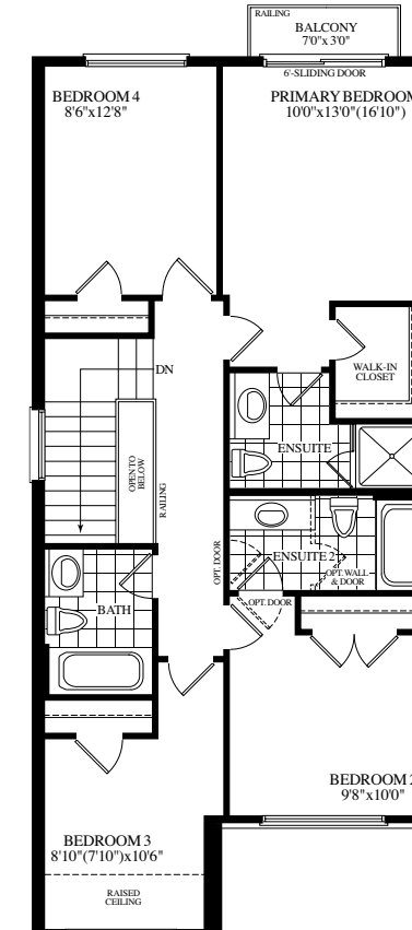
OPT. UPPER LEVEL ELEVATION A & B (4 BEDROOM)
