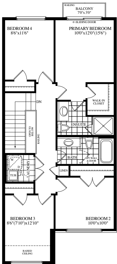
OPT. UPPER LEVEL ELEVATION A & B (4 BEDROOM)
