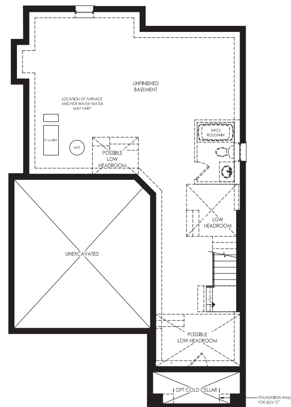
ALL ELEVATIONS BASEMENT
