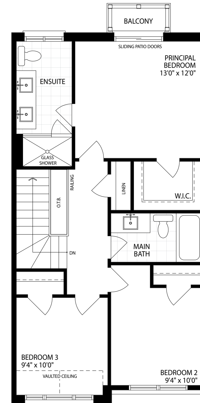
UPPER FLOOR ELEV. A
