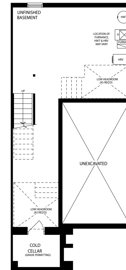
BASEMENT ELEV. A
