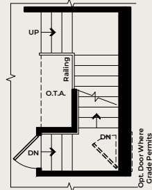
ALT. ENCLOSED STAIR LAYOUT
