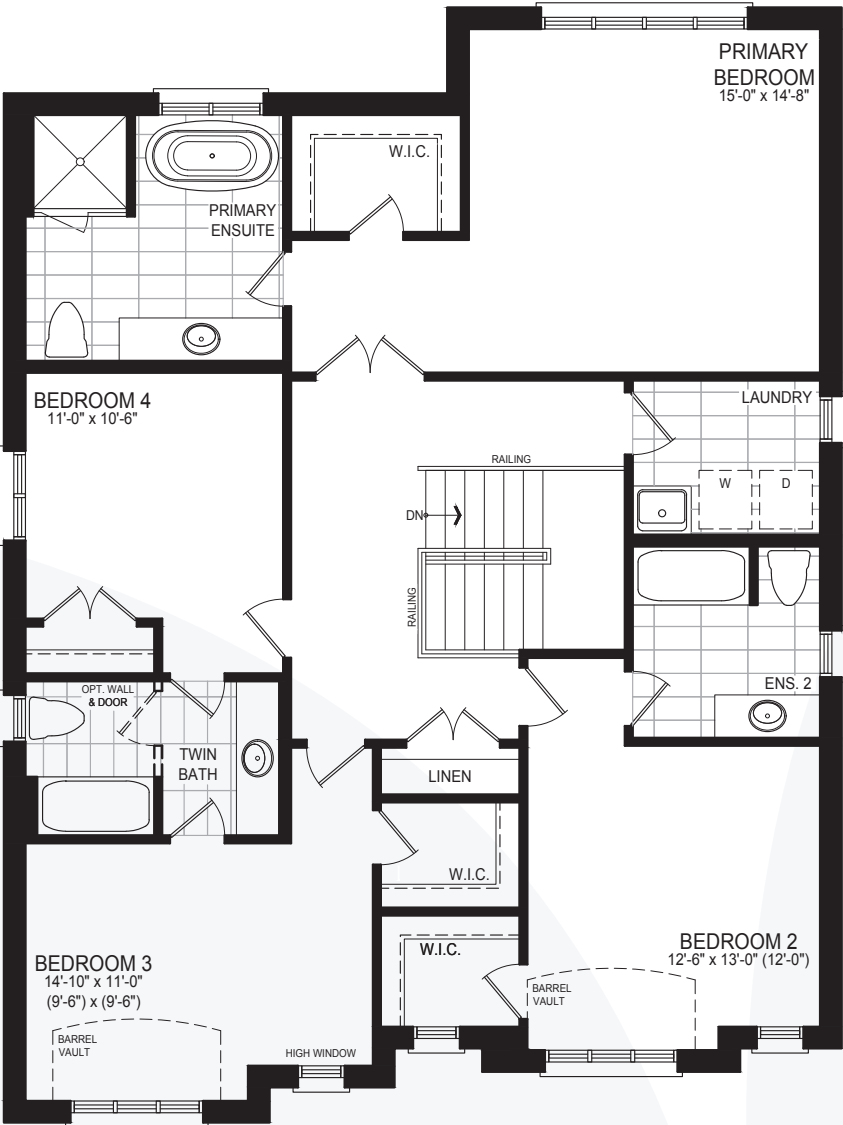
SECOND FLOOR Style B
