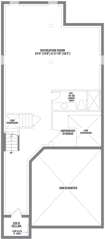
LOWER LEVEL ELEV. 'A', 'B' & 'C'
