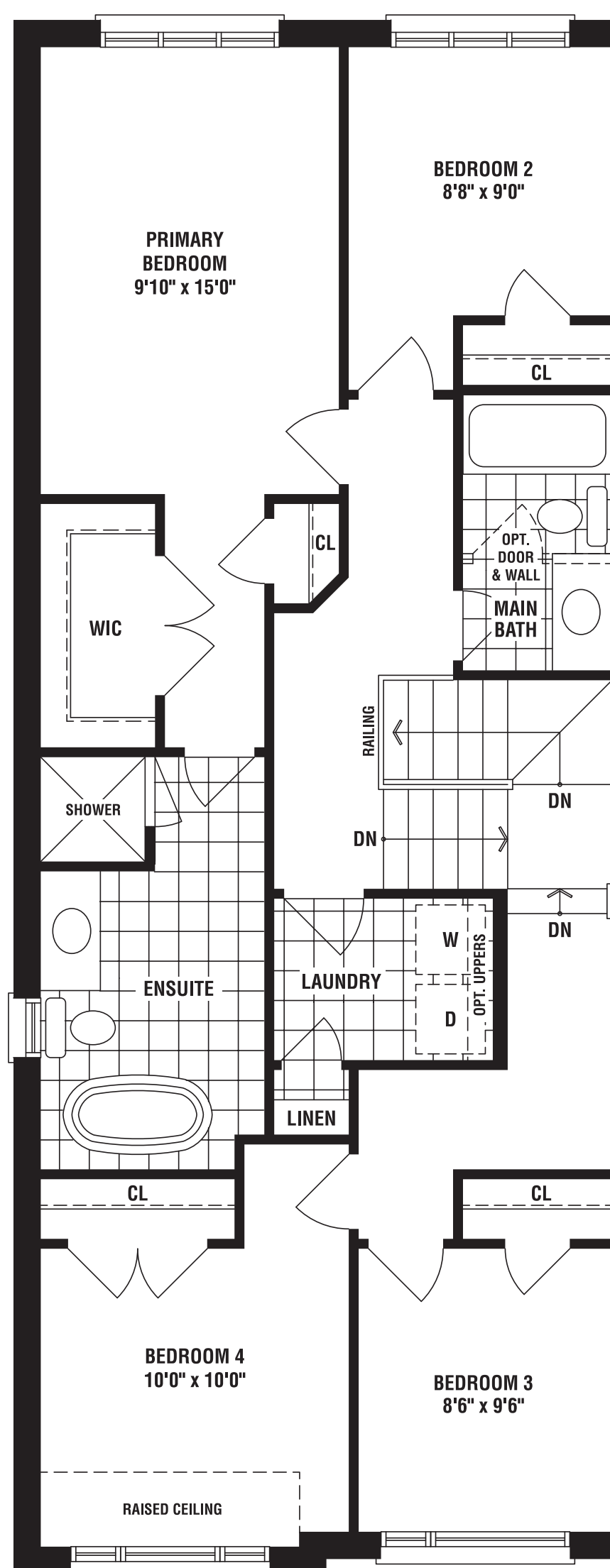
SECOND LEVEL PLAN ELEV. 'A1' END
