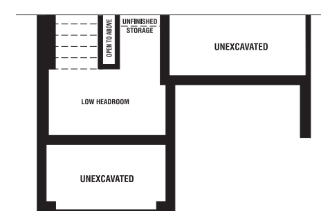
PARTIAL OPT. FINISHED LOWER LEVEL PLAN FILEV '81'
