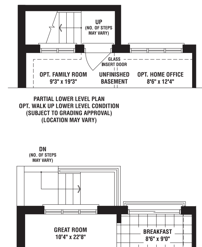
PARTIAL MAIN LEVEL PLAN OPT. WALK UP LOWER LEVEL CONDITION (SUBJECT TO GRADING APPROVAL) (LOCATION MAY VARY)
