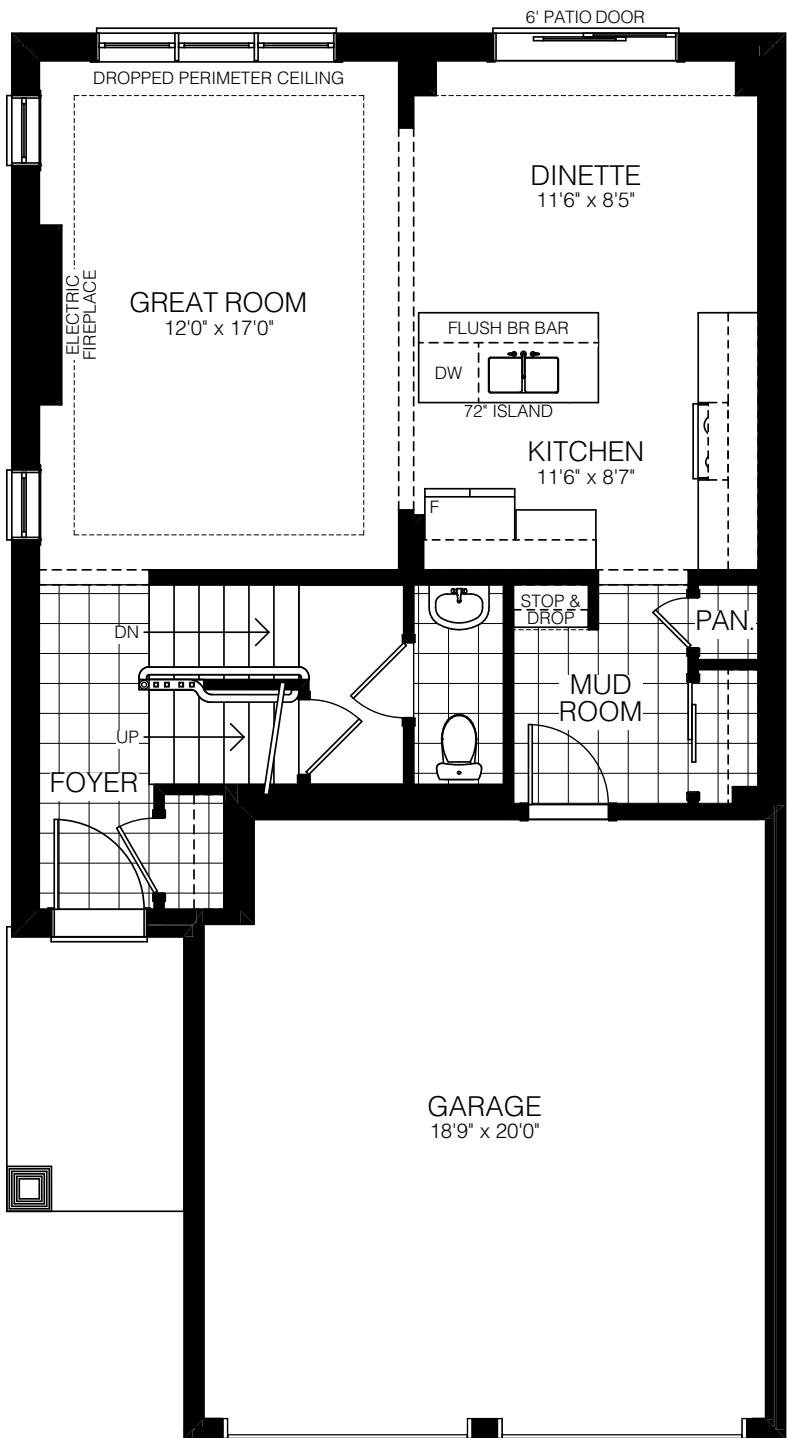
MAIN FLOOR ELEV. A
